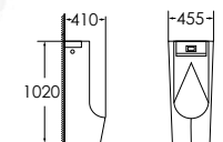
7001 Urinal Size: 455x410x1020 mm Fixing to wall with back
