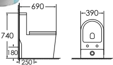
8214CKB Washdown one-piece toilet Size:690x390x740 mm P-trap,180mm roughing-in S-trap,250mm roughing-in Color:Calaeatta + Sky Blue
