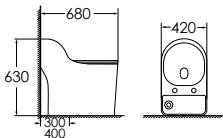
8205DBG Siphonic one-piece toilet Size: 680x420x630 mm S-trap, 300/400mm roughing-in
