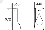
7003 Urinal Size: 440x365x970 mm Fixing to wall with back
