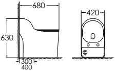
8205GR Siphonic one-piece toilet Size: 680x420x630 mm S-trap, 300/400mm roughing-in
