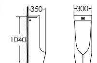
7033 Urinal Size: 300x350x1040 mm Fixing to wall with back
