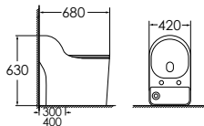
8205AG Siphonic one-piece toilet Size: 680x420x630 mm S-trap, 300/400mm roughing-in
