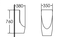
7009 Urinal Size: 350x380x760 mm Fixing to wall with back
