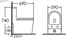
8214GW Washdown one-piece toilet Size:690x390x740 mm P-trap,180mm roughing-in S-trap,250mm roughing-in Color:Golden Line + White
