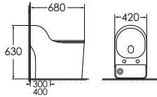
8205PM Siphonic one-piece toilet Size: 680x420x630 mm S-trap, 300/400mm roughing-in
