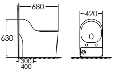
8205OG Siphonic one-piece toilet Size: 680x420x630 mm S-trap, 300/400mm roughing-in
