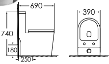
8214CBM Washdown one-piece toilet Size:690x390x740 mm P-trap,180mm roughing-in S-trap,250mm roughing-in Color:Calaeatta + Black Matt
