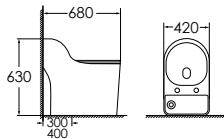
8205WG Siphonic one-piece toilet Size: 680x420x630 mm S-trap, 300/400mm roughing-in
