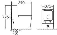
8108 Siphonic one-piece toilet Size:690x375x775 mm S-trap,300/400mm roughing-in
