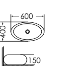
XS-0031B Art basin Size: 600x400x150 mm Above counter mounting
