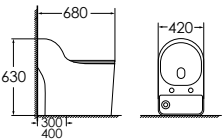
8205GG Siphonic one-piece toilet Size: 680x420x630 mm S-trap, 300/400mm roughing-in
