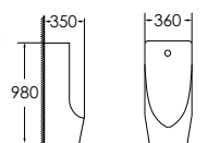
7006 Urinal Size: 360x350x980 mm Fixing to wall with back
