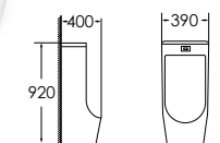
7032 Urinal Size: 390x400x1000 mm Fixing to wall with back
