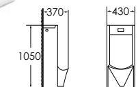
7004 Urinal Size: 430x370x1050 mm Fixing to wall with back
