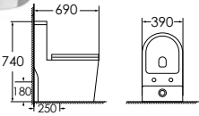
8214CGM Washdown one-piece toilet Size:690x390x740 mm P-trap,180mm roughing-in S-trap,250mm roughing-in Color:Calaeatta + Grey Matt
