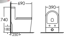
8214CPM Washdown one-piece toilet Size:690x390x740 mm P-trap,180mm roughing-in S-trap,250mm roughing-in Color:Calaeatta + Pink Matt
