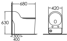
8205BG Siphonic one-piece toilet Size: 680x420x630 mm S-trap, 300/400mm roughing-in
