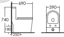
8214PW Washdown one-piece toilet Size:690x390x740 mm P-trap,180mm roughing-in S-trap,250mm roughing-in Color:Purple Line + White
