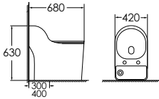
8205DB Siphonic one-piece toilet Size: 680x420x630 mm S-trap, 300/400mm roughing-in
