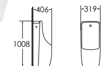
7035 Urinal Size: 319x406x1008 mm Fixing to wall with back
