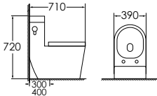
8076 Siphonic one-piece toilet Size:710x390x720 mm S-trap,300/400mm roughing-in
