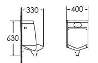
7012 Urinal Size: 400x330x630 mm Fixing to wall with back
