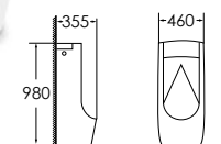
7005 Urinal Size: 460x355x980 mm Fixing to wall with back
