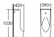
7034 Urinal Size: 390x420x1030 mm Fixing to wall with back
