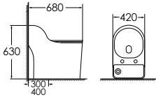
8205B Siphonic one-piece toilet Size: 680x420x630 mm S-trap, 300/400mm roughing-in
