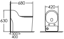
8205OR Siphonic one-piece toilet Size: 680x420x630 mm S-trap, 300/400mm roughing-in
