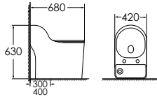
8205AT Siphonic one-piece toilet Size: 680x420x630 mm S-trap, 300/400mm roughing-in
