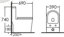
8214BW Washdown one-piece toilet Size:690x390x740 mm P-trap,180mm roughing-in S-trap,250mm roughing-in Color:Blue Line + White
