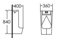
7011 Urinal Size: 360x400x840 mm Fixing to wall with back
