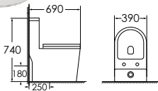
8214BLW Washdown one-piece toilet Size:690x390x740 mm P-trap,180mm roughing-in S-trap,250mm roughing-in Color:Black Line + White
