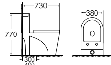
8018 Siphonic one-piece toilet Size: 730x380x770 mm S-trap, 300/400mm roughing-in
