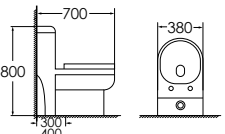
8010 Siphonic one-piece toilet Size: 700x380x800 mm S-trap, 300/400mm roughing-in
