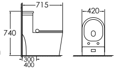
8112 Siphonic one-piece toilet Size: 715x420x740 mm S-trap, 300/400mm roughing-in
