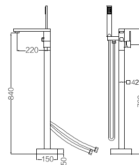
DT-1120 落地式浴缸淋浴龙头 Bath shower floor standing mixer 材料 /Material: A 级铜 /Brass
