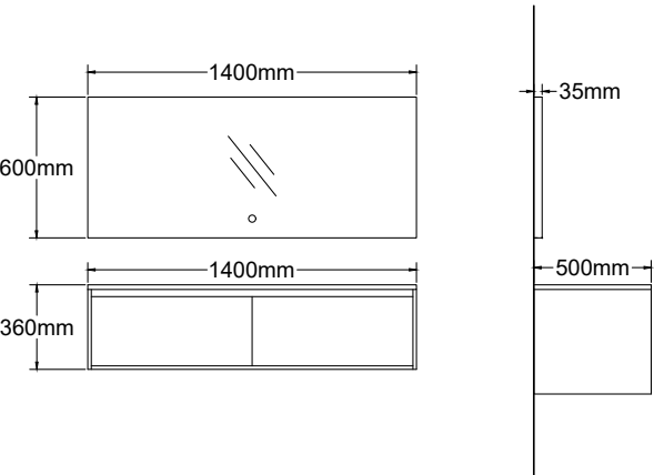
F-5072 LED 主柜 /Main Cabinet : 1400x500 mm 镜子 /Mirror : 1400x600 mm 岩板 /Sintered Stone : Arabescato Corchia 材质 /Plywood
