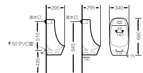
7015 Wall hung urinal Size:340x295x680mm Fixing to wall with back
