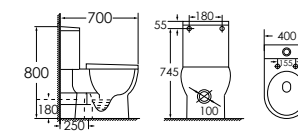
1023A Washdown two-piece toilet Size: 700x400x800 mm P-trap, 180 mm roughing-in S-trap, 250 mm roughing-in
