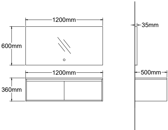
F-5073 LED 主柜 /Main Cabinet : 1200x500 mm 镜子 /Mirror : 1200x600 mm 岩板 /Sintered Stone : Arabescato Corchia 材质 /Plywood
