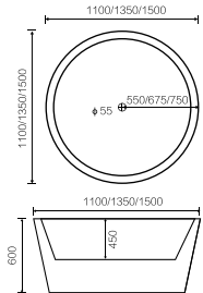
BT-054 独立式浴缸 Freestanding bathtub 尺寸 /Size: 1100x1100x600 mm 1350x1350x600 mm 1500x1500x600 mm
