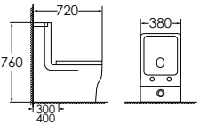
8096 Siphonic one-piece toilet Size: 720x380x760 mm S-trap, 300/400mm roughing-in
