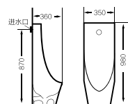
7006 Floor standing urinal Size:350x360x980 mm Back to wall installation
