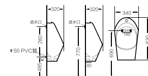
7025 Wall hung urinal Size:340x320x630mm Fixing to wall with back
