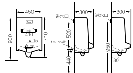
7013 Wall hung urinal Size:450x300x710 mm Fixing to wall with back
