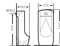
7003 Floor standing urinal Size:443x373x1000 mm Back to wall installation
