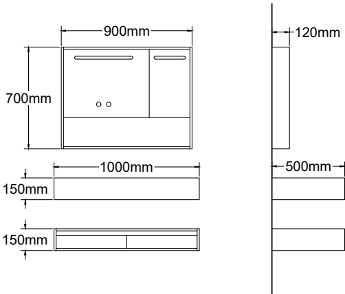
F-5076 F-5077 LED Main Cabinet: 1000x500mm Countertops: 1000x500mm Mirror Cabinet: 900x700mm Sintered Stone: Arabescato Corchia
