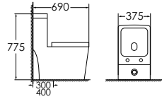
8108 Siphonic one-piece toilet Size: 690x375x775 mm S-trap, 300/400mm roughing-in
