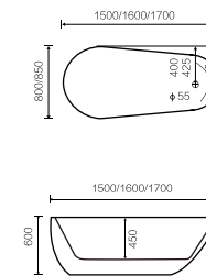
BT-020 独立式浴缸 Freestanding bathtub 尺寸 /Size: 1500x800x600 mm 1600x800x600 mm 1700x850x600 mm
