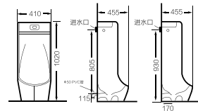
7001 Floor standing urinal Size:410x455x1020 mm Back to wall installation
